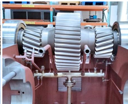
Combiflex gearbox refurbishment in the South Africa Service Center
